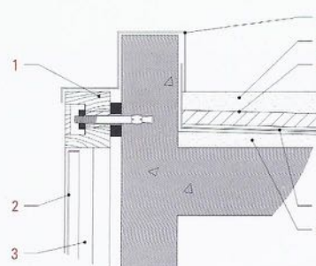
roof & facade detail C
