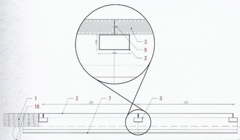
facade horizontal section detail
