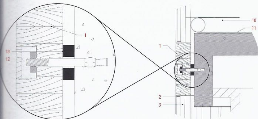
facade detail B
