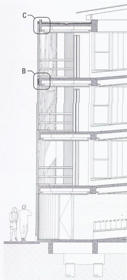
partial section A
