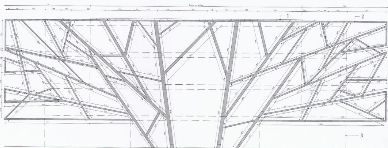
facade development figure - laminated wood beams geometry
